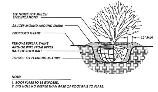
3 L2.0 DECIDUOUS SHRUB PLANTING DETAIL N.T.S.
